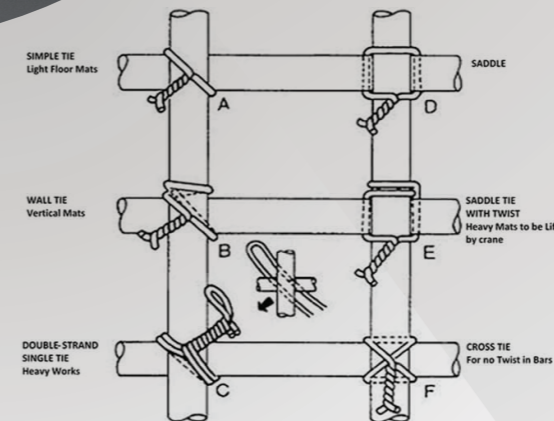
6 WAYS OF TYING BINDING WIRE
